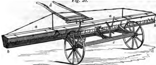
A MACHINE FOR SOWING CORN BROADCAST UPON THE GROUND.
